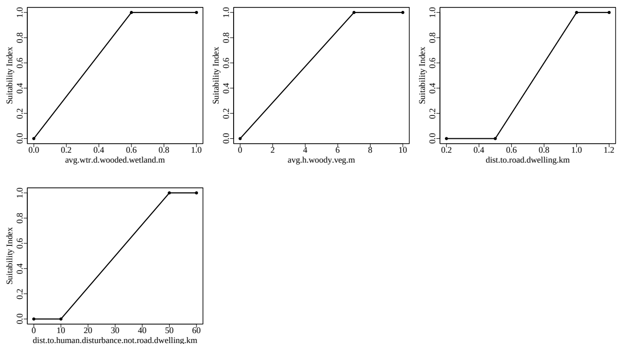
Figure 1. Suitability index graphs for variables included in the grete-gretNestingNonisland model in ecorest .
